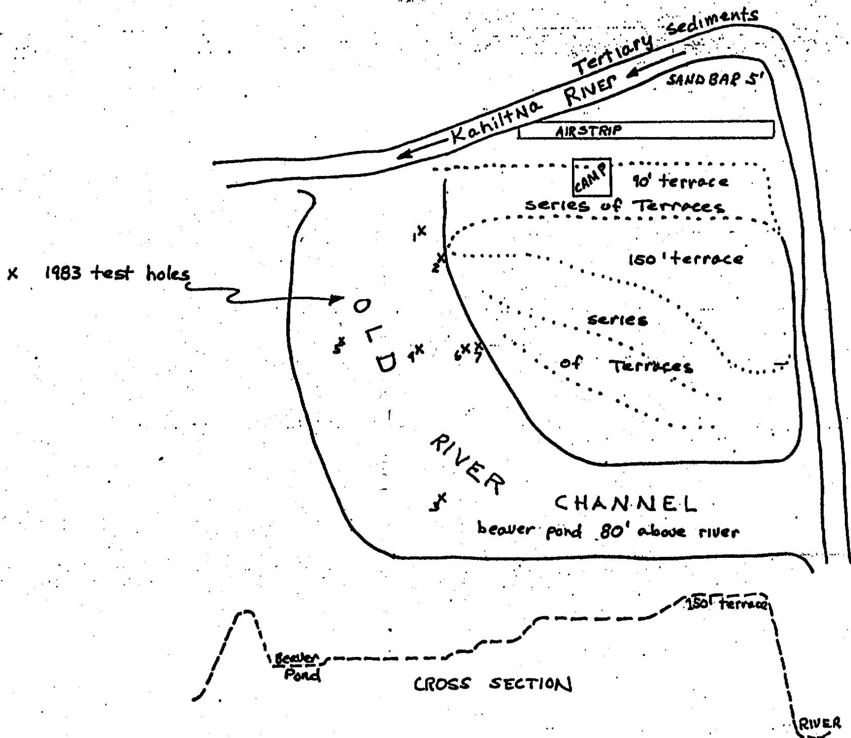
Figure 4. Sketch of the airstrip, camp, test pits, existing mine area and proposed mine area. The airstrip is 1240 feet long and can be used as a scale.
